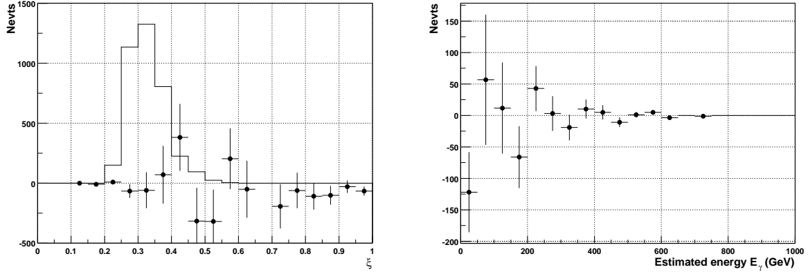
Fig. 3. Left: On-Off distribution of \xi for M31 data (2001-03, black markers with error bars), with respect to the same simulated spectrum as figure 2-left (solid line). Right: On-Off distribution of the estimated energy for all events within analysis cuts.
